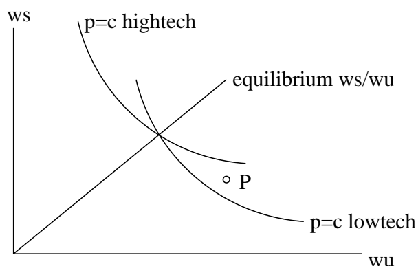
Mussa diagram: zero profit lines
